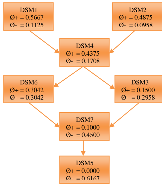
Figure 1 Visual computation of the total net flow using PROMETHEE I
