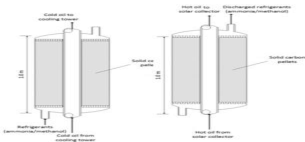
From left: Figure 7(a) Adsorber model in charging mode, Figure 7(b) Adsorber model in discharging mode
