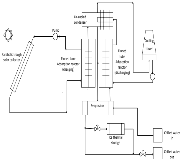
Figure 5 Adsorption chillers with ice production thermal storage
