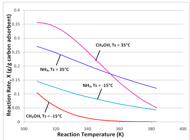
Figure 6 Adsorption capacity for system with ice thermal storage
