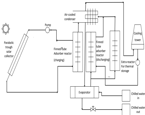
Figure 4 Adsorption chillers with extended capacity adsorber beds
