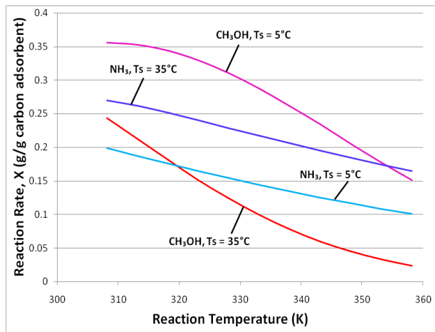
Figure 2 Calculated adsorption capacity of ammonia and methanol for hot water thermal storage
