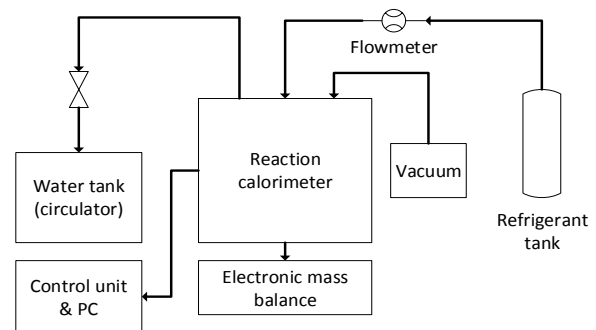
Figure 8 Reaction calorimetry experimental set up.
