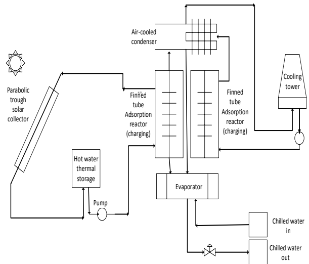
Figure 3 Adsorption chillers with hot water thermal storage
