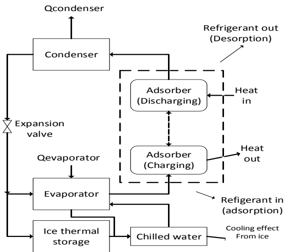
Figure 1 Solar adsorption refrigeration system
