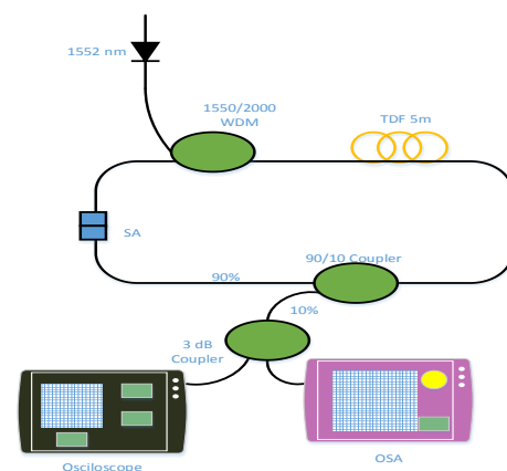
Figure 1 Experimental setup of Q-switched TDFL with 1552 nm pump
