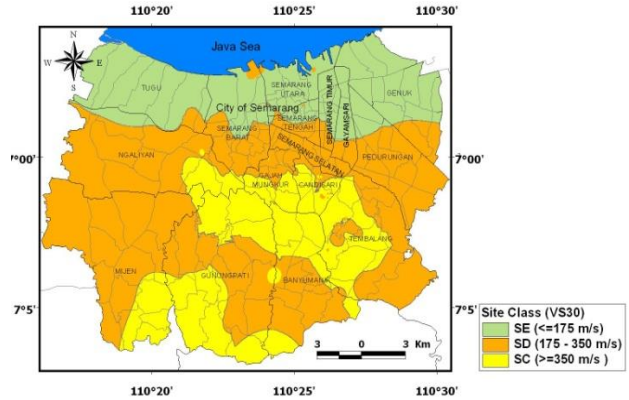
Figure 4 Site classification of Semarang using V_{s30} value
