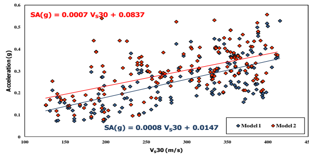
Figure 12 PGA at Ground Surface calculated at 190 points for Model 1 and Model 2
