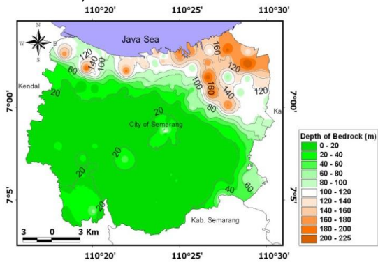
Figure 3 Contour map of depth of engineering bedrock identified by single station feedback seismometer Site characterization (classification) was carried out by interpreting the results of field measurements including in-situ standard penetration test (SPT) and laboratory tests, following the same method used by
