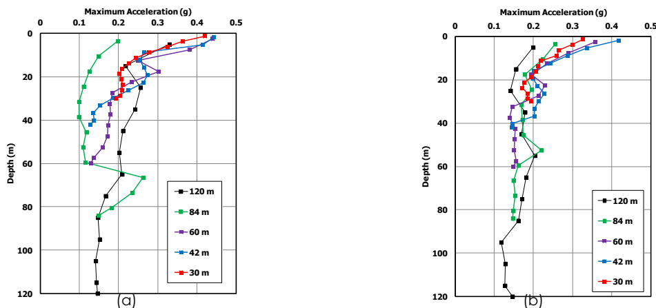
Figure 9 Maximum acceleration profiles for (a) clay and (b) sand
