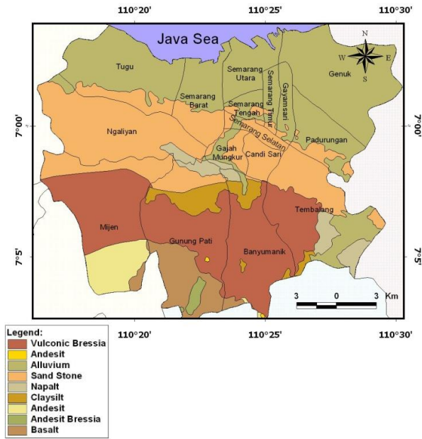
Figure 2 Geological map of Semarang, modified from [8]
