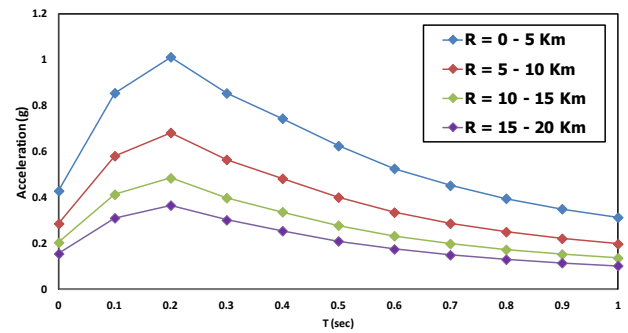
Figure 5 Target spectrum used for spectral matching analysis
