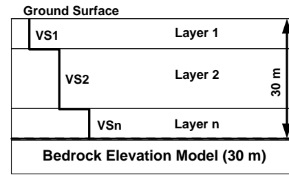
Figure 8 Model 2 for site response analysis
