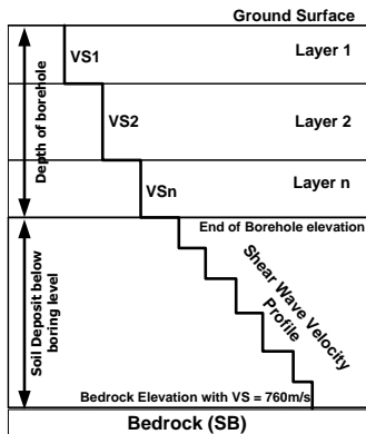
Figure 7 Model 1 for site response analysis
