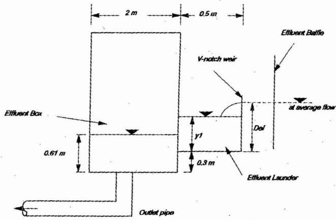
(a) Detail of Effluent Structure and Hydraulic Profile
