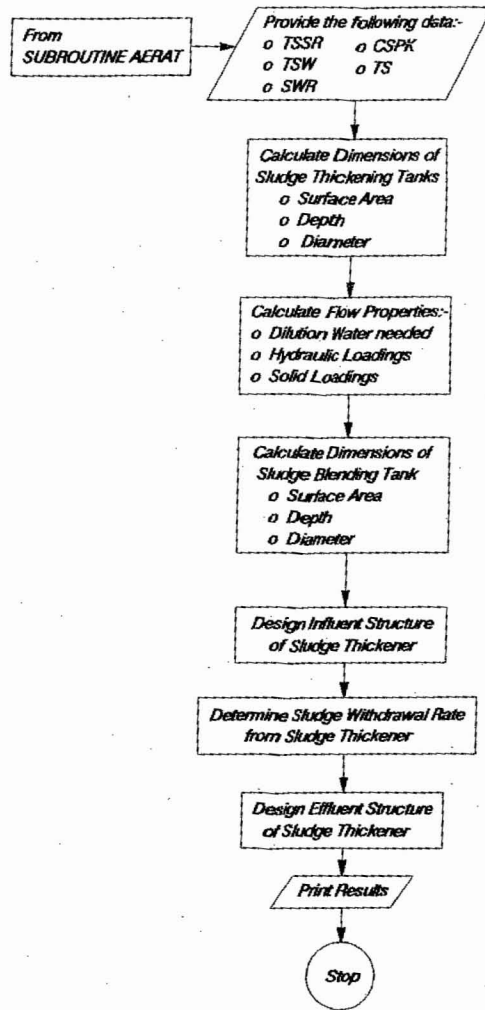
FIGURE 5 : FLOWCHART FOR THE DESIGN OF SLUDGE THICKENER AND SLUDGE BLENDING TANK (SUBROUTINE THICK)
