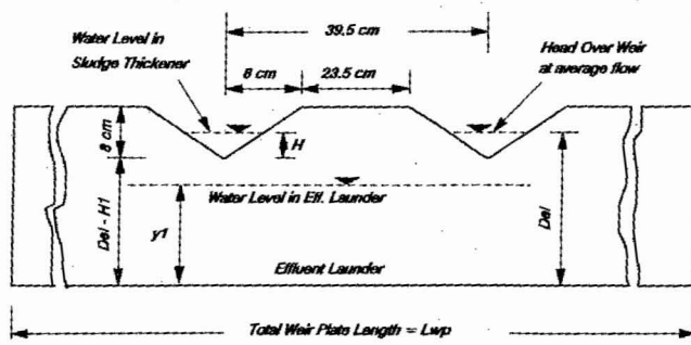
(b) Detail of Weir Plate and V-notches
