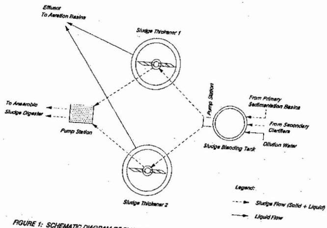
FIGURE 1: SCHEMATIC DIAGRAM OF SLUDGE BLENDING TANK AND GRAVITY THICKENER
