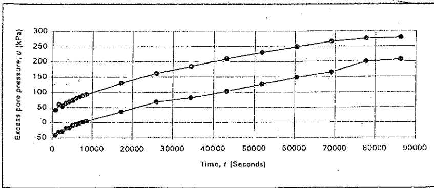
(c) q_c/p'_e = 0.256
