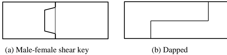
Figure 2: Precast panel dry joints
