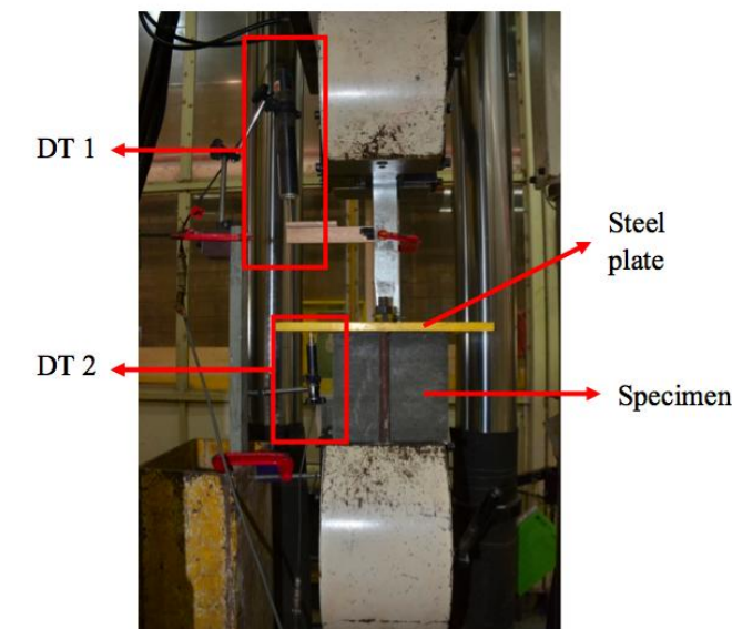
Figure 6: The test setup of the pull-out test.
