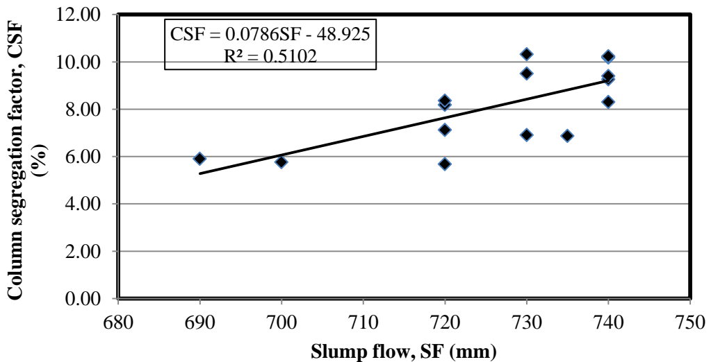
Figure 7: Correlation between slump flow and column segregation factor
