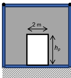
Figure 3 SPSW model with different height of perforation.
